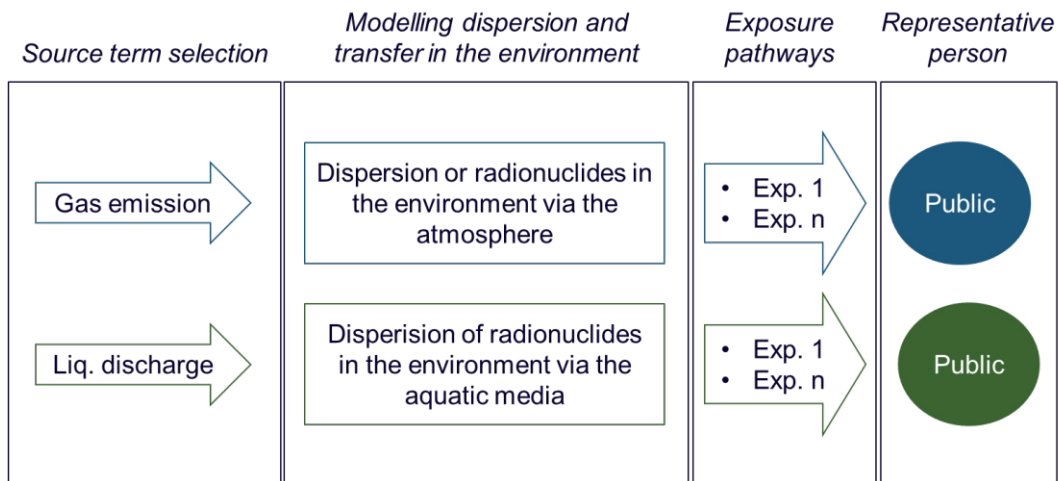
Figure 3-2. Conceptual model scheme for human dose assessment from IFE Kjeller's plants discharges.
