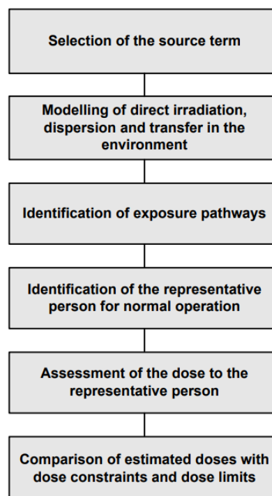
Figure 3-1. Scheme showing the components of a radiological environmental impact assessment for protection of the public in normal operation [9].
