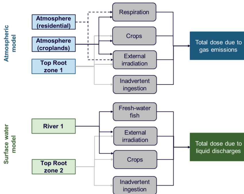
Figure 3-12. Relevant compartments for the estimation of the dose to public in the atmospheric and surface water model.
